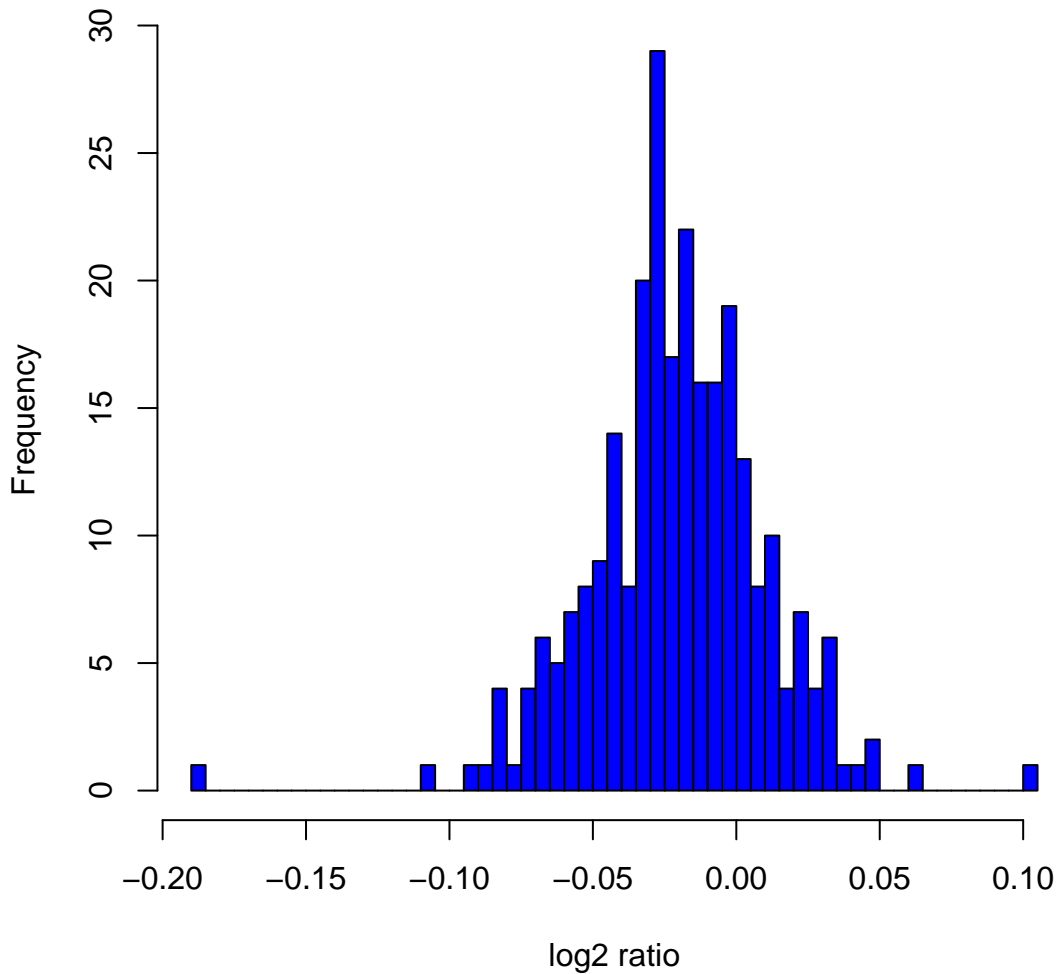
Histogram of log 2 ratios in 270 HapMap samples at clone Chr18tp-2E9
