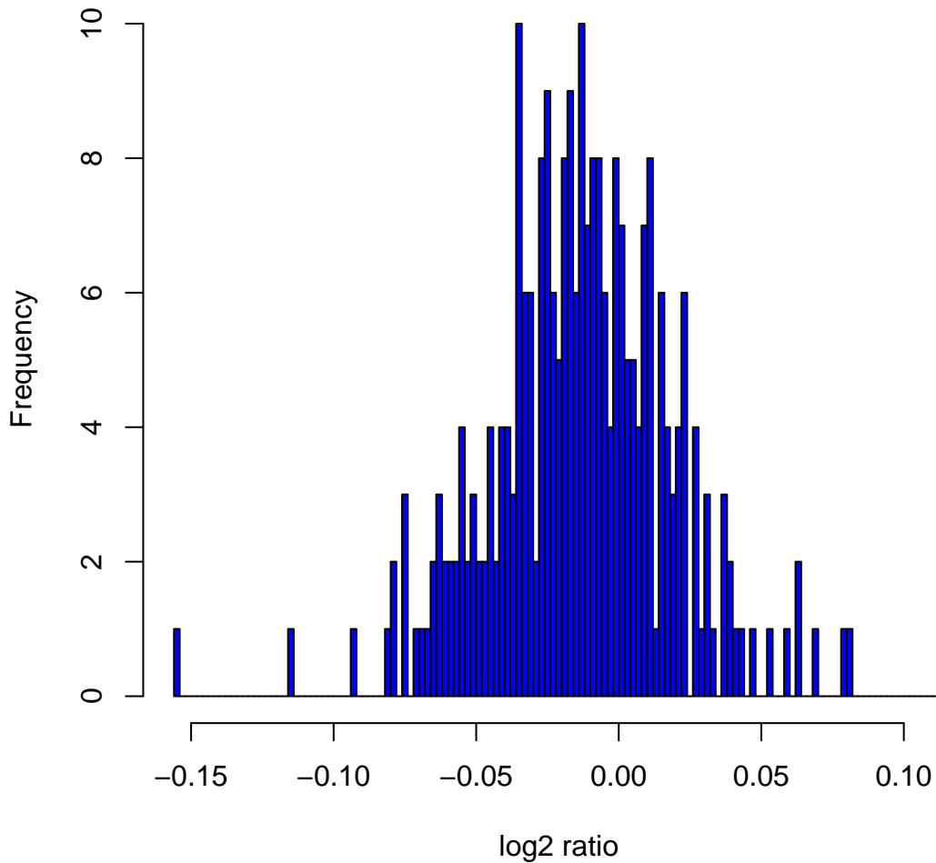
Histogram of log 2 ratios in 270 HapMap samples at clone Chr18tp-2G2
