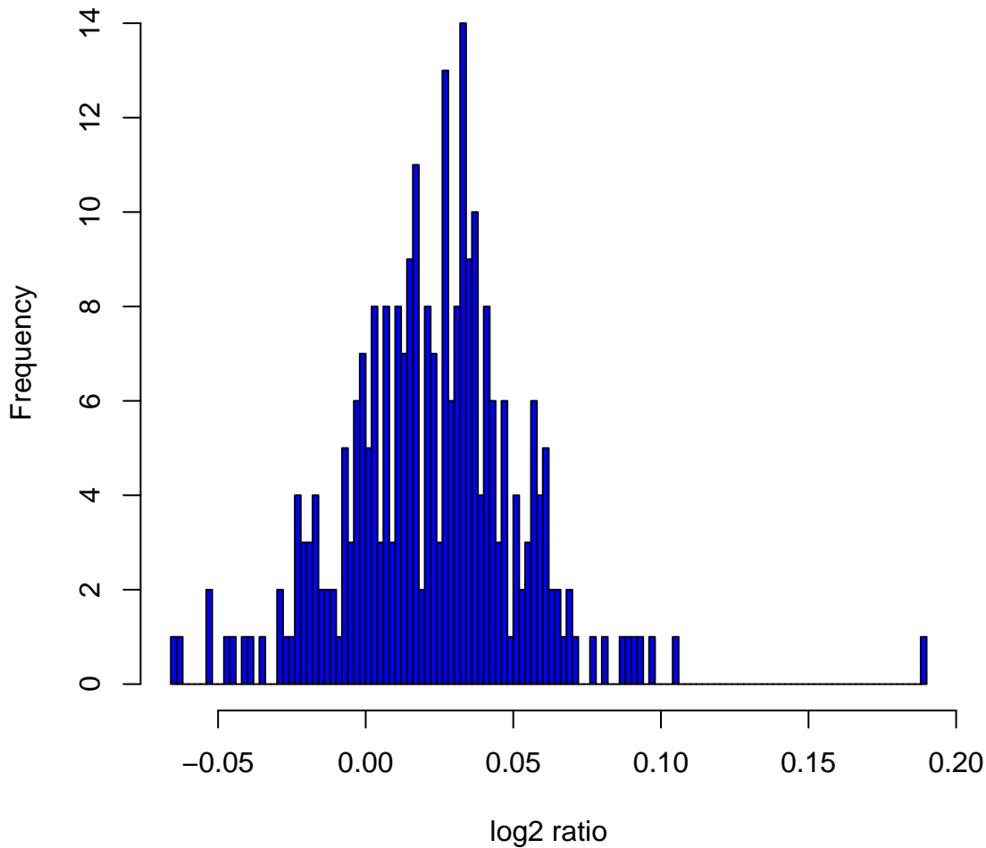
Histogram of log 2 ratios in 270 HapMap samples at clone Chr18tp-3A1
