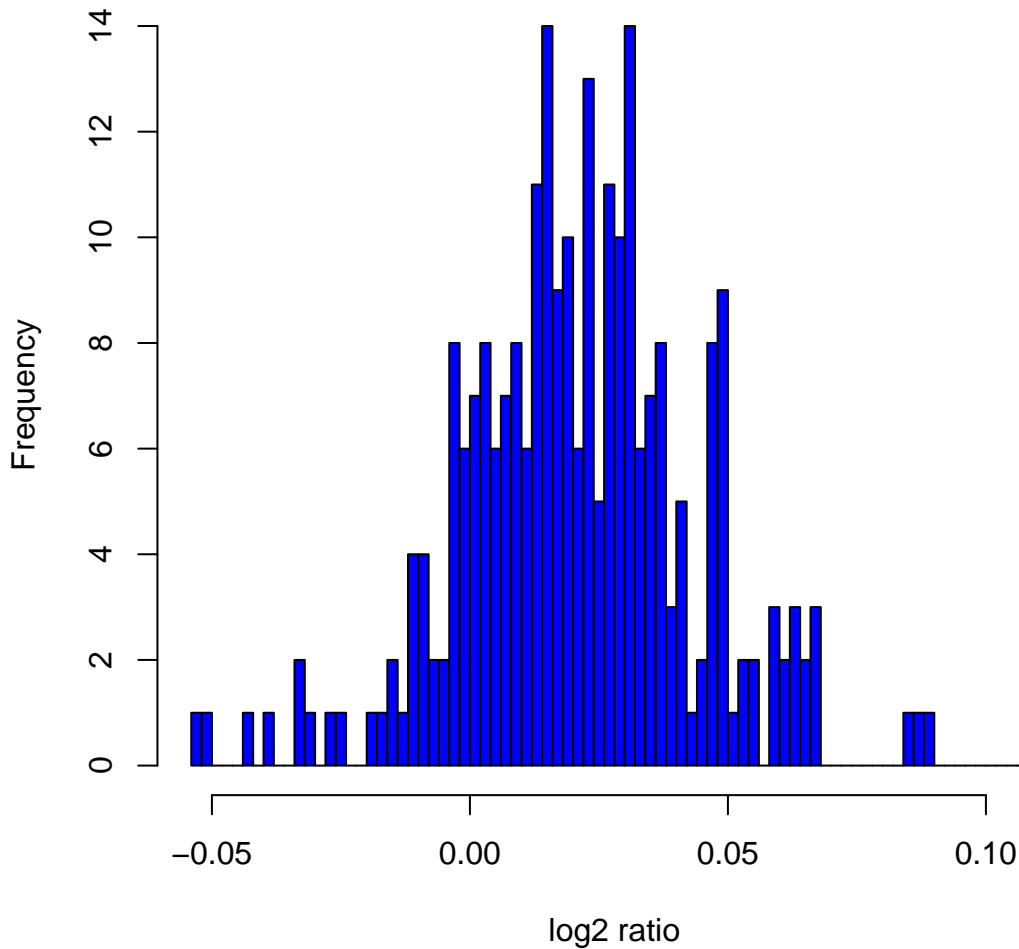
Histogram of log 2 ratios in 270 HapMap samples at clone Chr18tp-3B2
