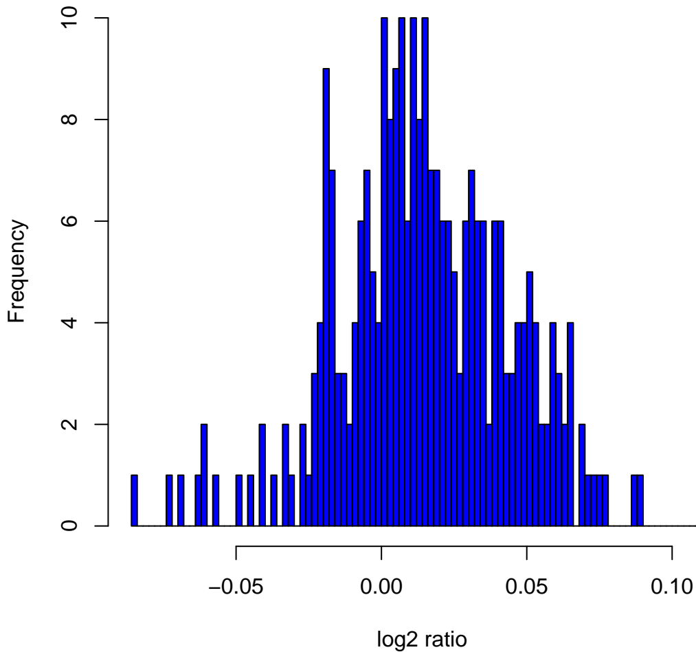
Histogram of \log_2 ratios in 270 HapMap samples at clone Chr18tp-3D4
