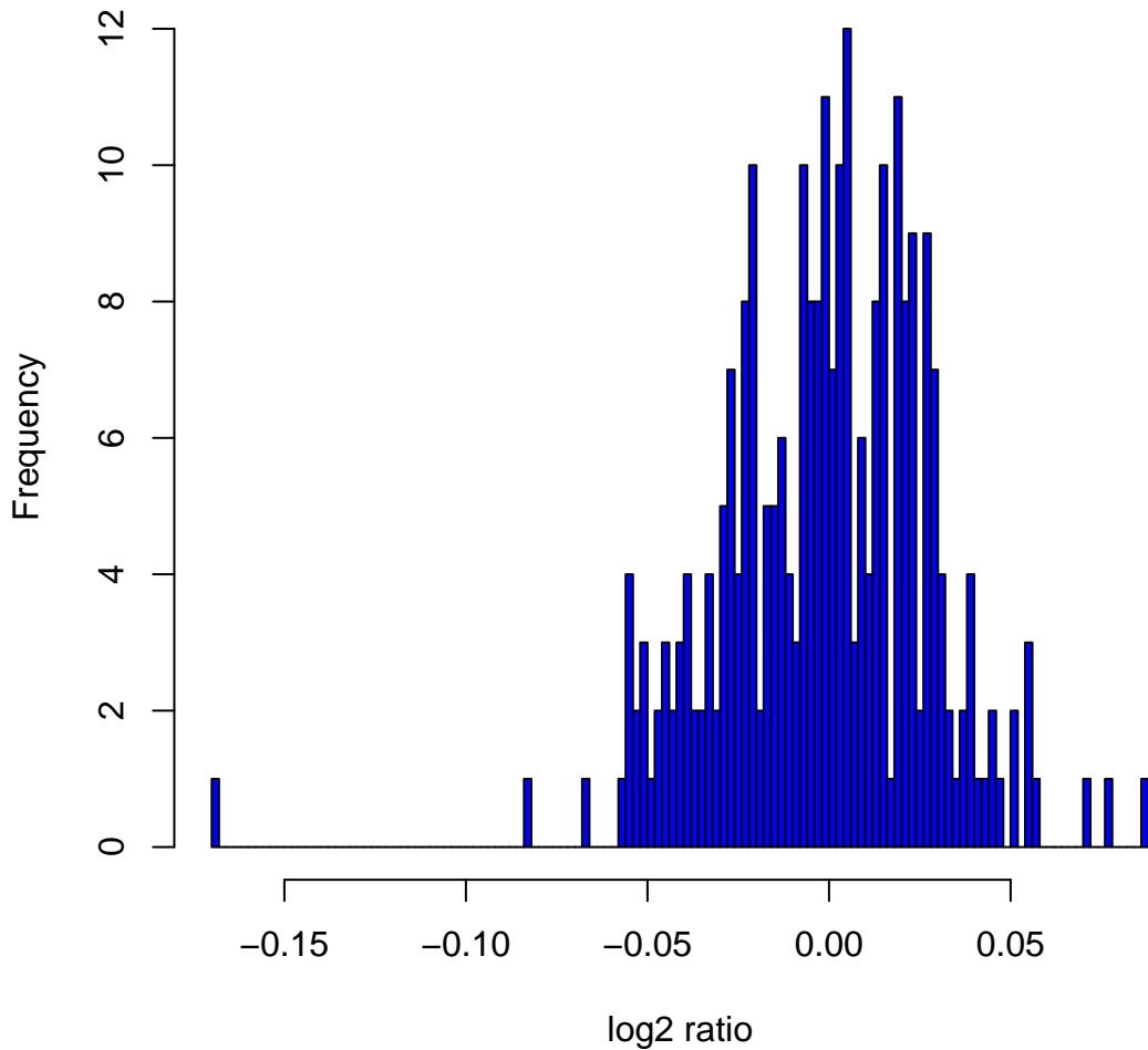
Histogram of log 2 ratios in 270 HapMap samples at clone Chr18tp-3E7
