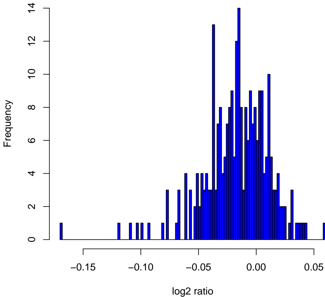
Histogram of log2ratios in 270 HapMap samples at clone Chr18tp-4A10
