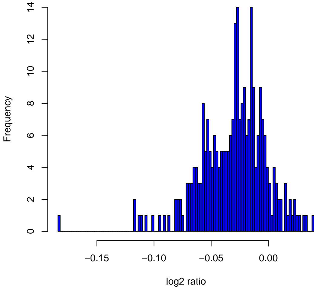
Histogram of log 2 ratios in 270 HapMap samples at clone Chr18tp-4D2
