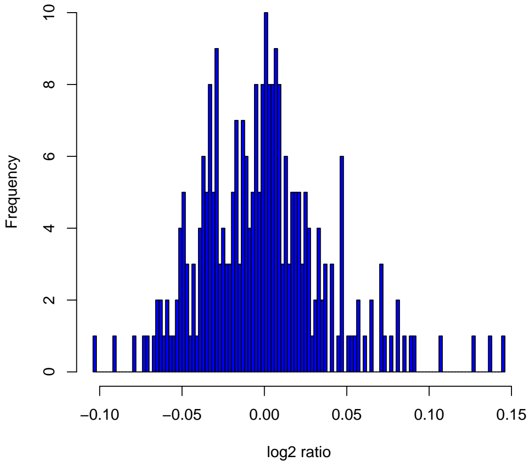
Histogram of log2ratios in 270 HapMap samples at clone Chr18tp-4G11
