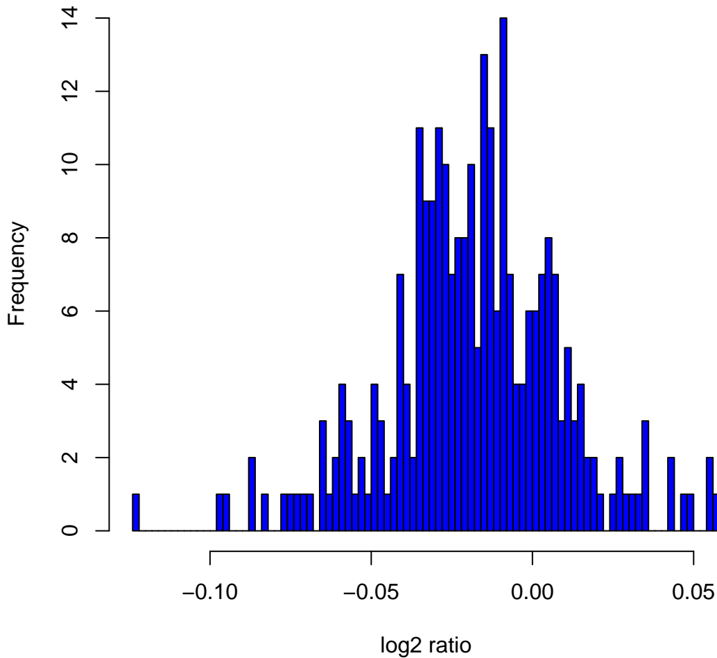
Histogram of log 2 ratios in 270 HapMap samples at clone Chr18tp-5C4
