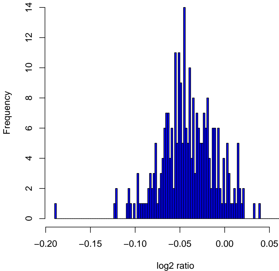
Histogram of log 2 ratios in 270 HapMap samples at clone Chr18tp-5D6
