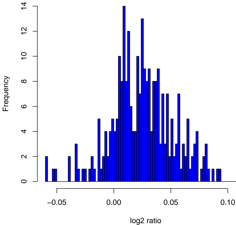
Histogram of log2ratios in 270 HapMap samples at clone Chr18tp-5F12
