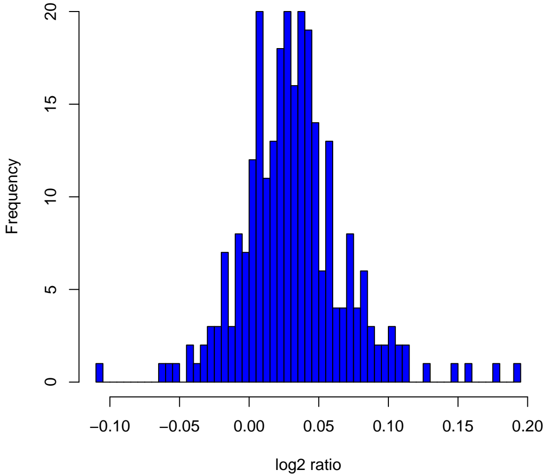
Histogram of log 2 ratios in 270 HapMap samples at clone Chr18tp-6C3
