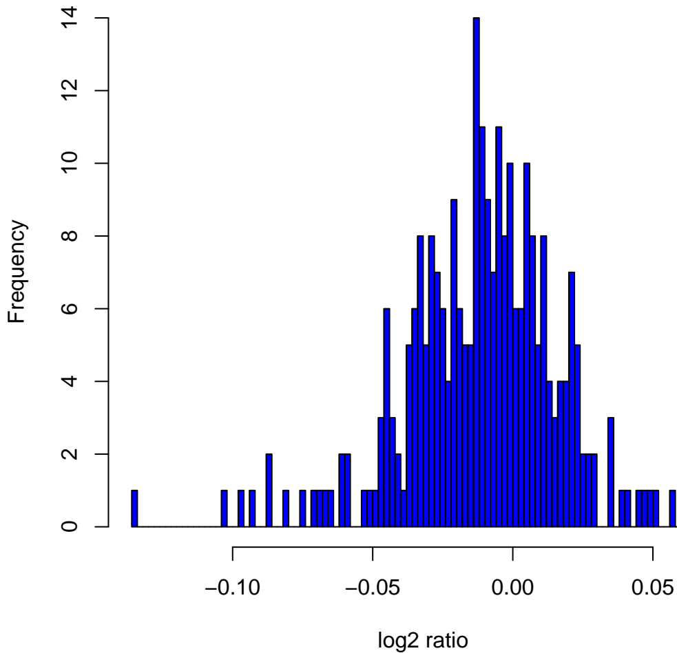
Histogram of log2ratios in 270 HapMap samples at clone Chr18tp-8C9
