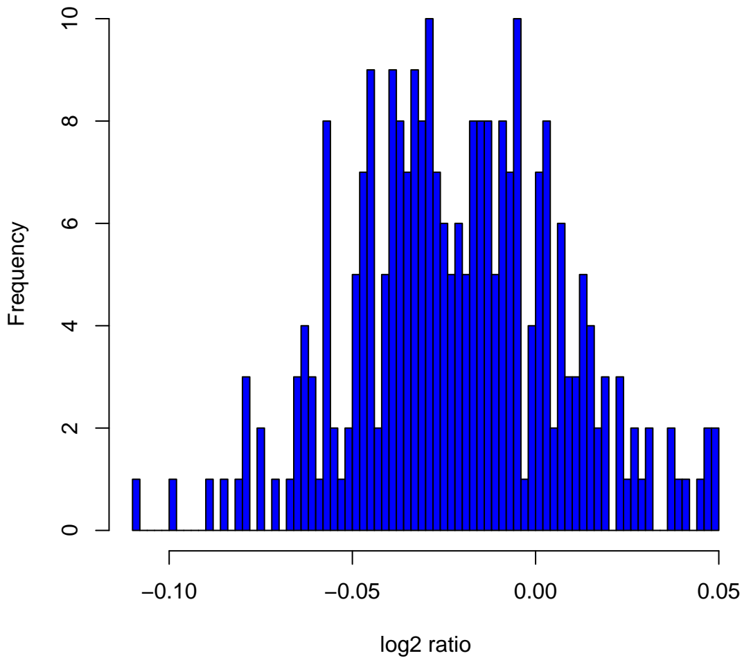
Histogram of log2ratios in 270 HapMap samples at clone Chr18tp-8D2
