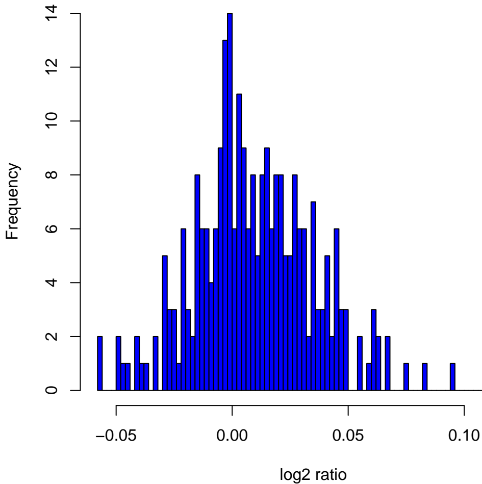
Histogram of log 2 ratios in 270 HapMap samples at clone Chr18tp-8D3
