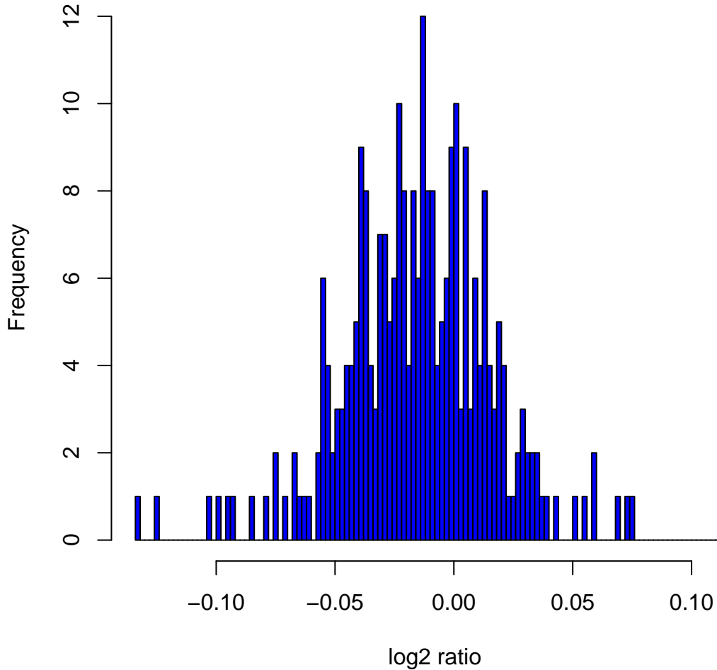
Histogram of \log_2 ratios in 270 HapMap samples at clone Chr18tp-8G8
