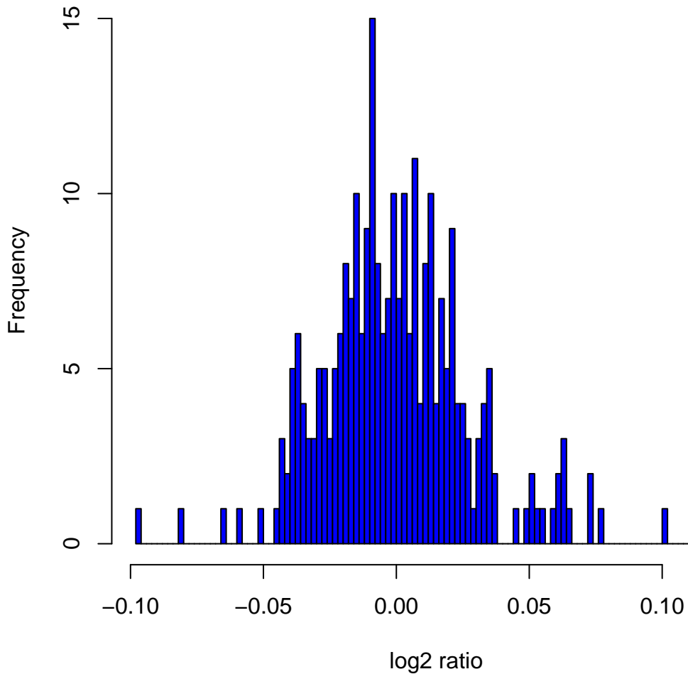
Histogram of log 2 ratios in 270 HapMap samples at clone Chr18tp-9B1
