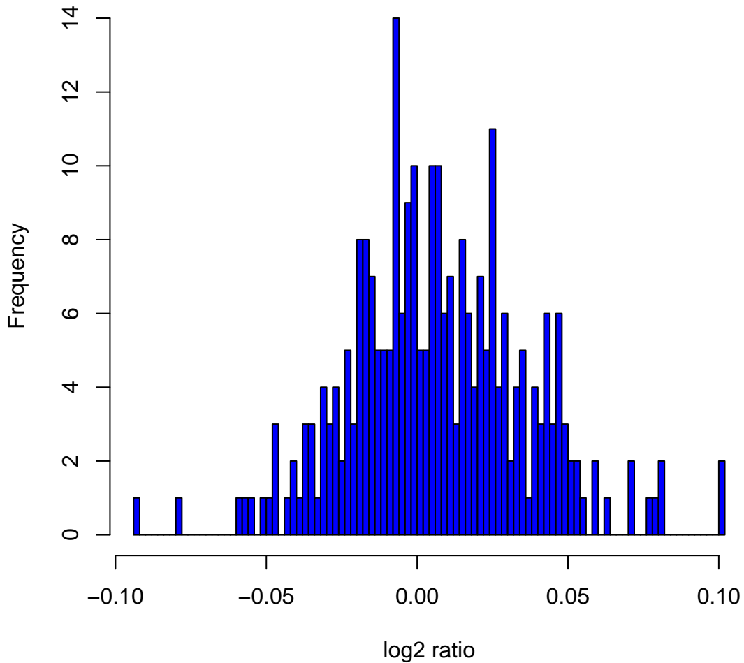
Histogram of log2ratios in 270 HapMap samples at clone Chr18tp-9E10
