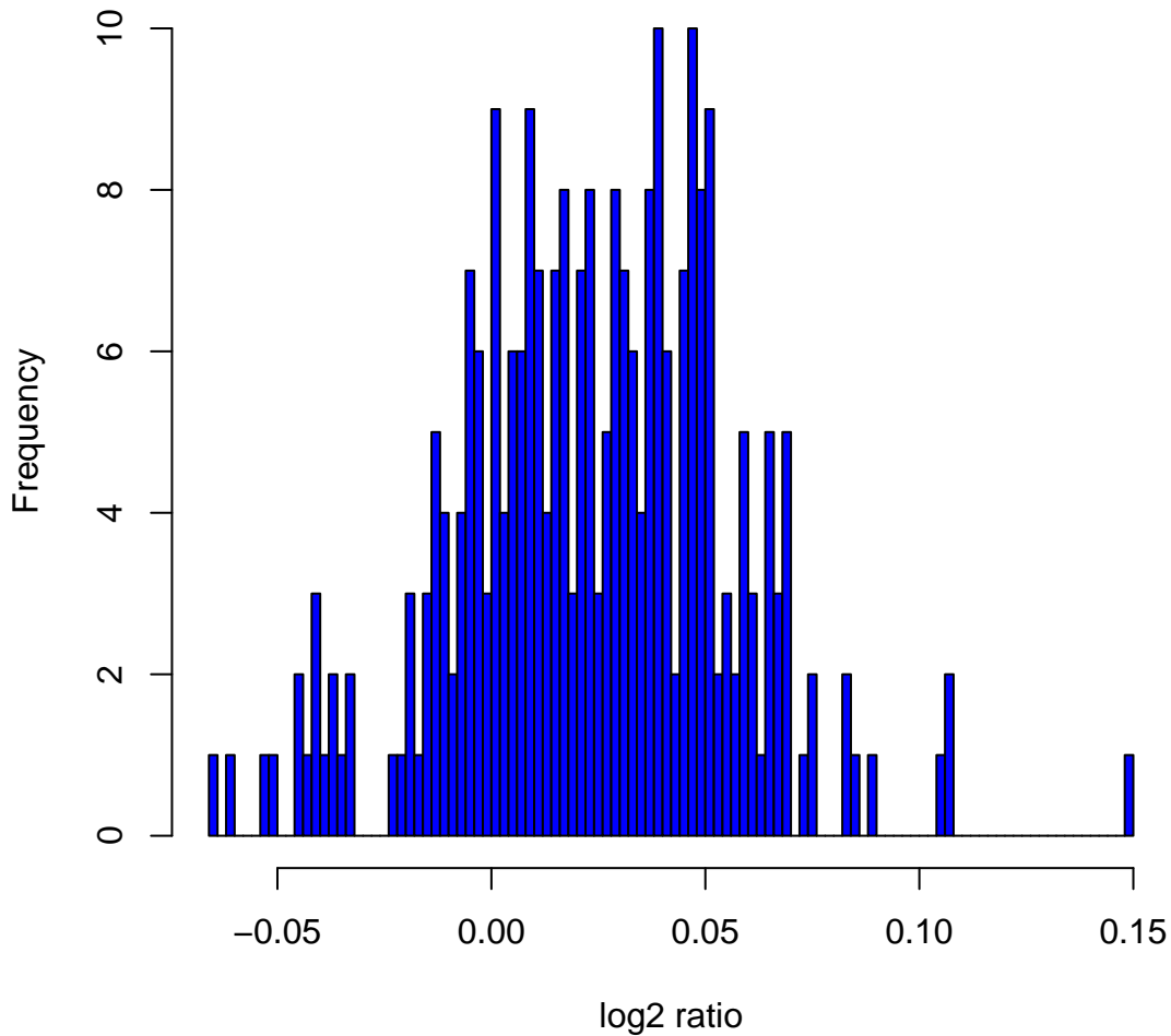
Histogram of log 2 ratios in 270 HapMap samples at clone Chr18tp-9G2
