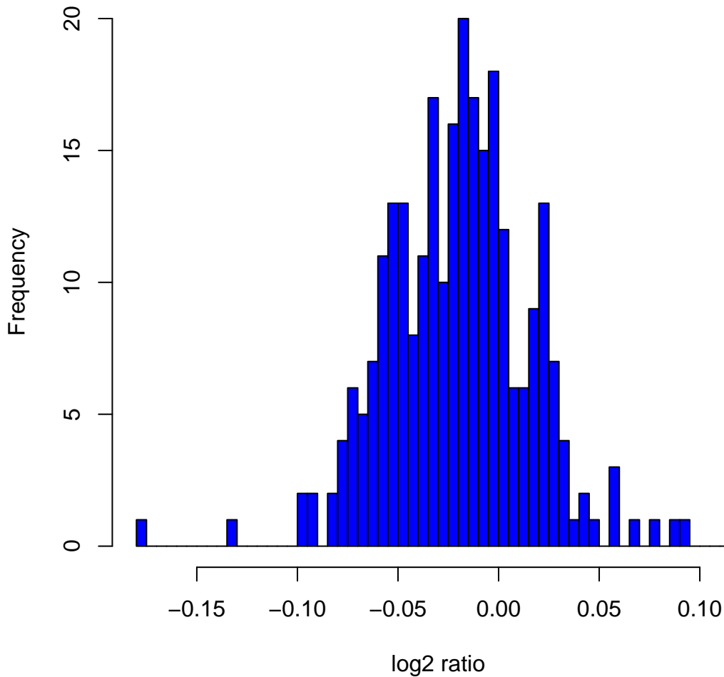
Histogram of log 2 ratios in 270 HapMap samples at clone Chr18tp-9G3
