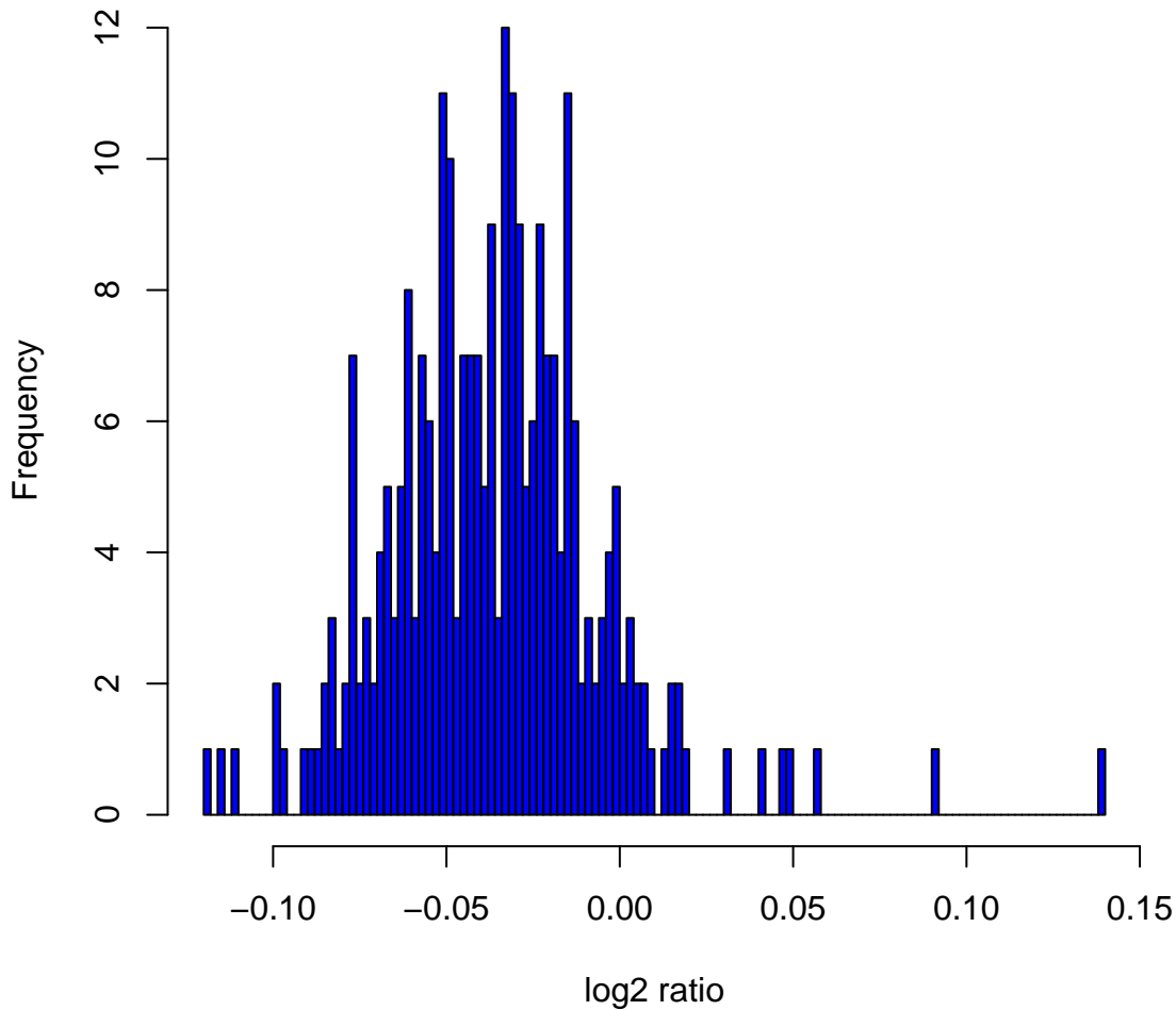
Histogram of \log_2 ratios in 270 HapMap samples at clone Chr18tp-9G8
