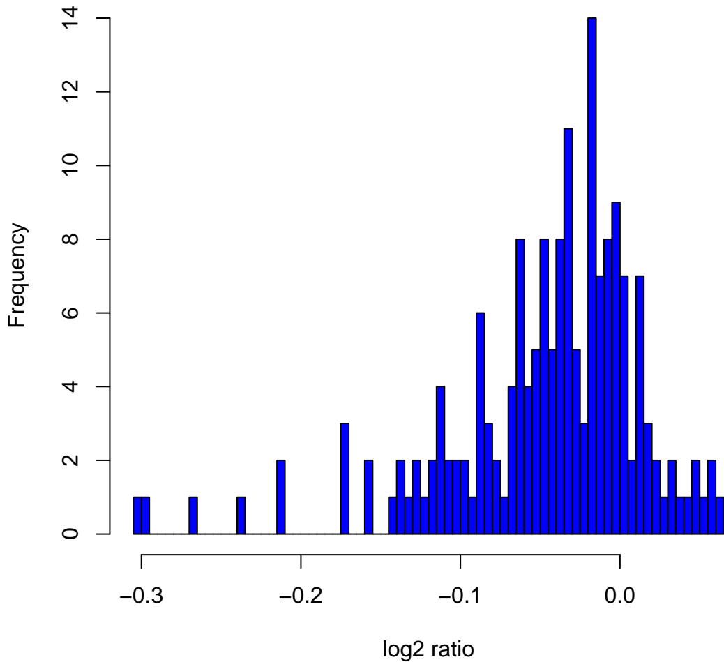
Histogram of log2ratios in 270 HapMap samples at clone Chr18tp-9H10
