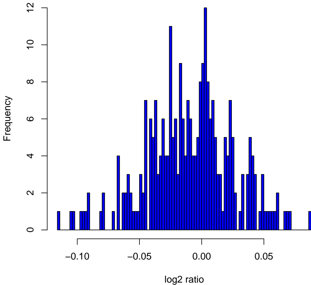
Histogram of log 2 ratios in 270 HapMap samples at clone Chr18tp-9H4
