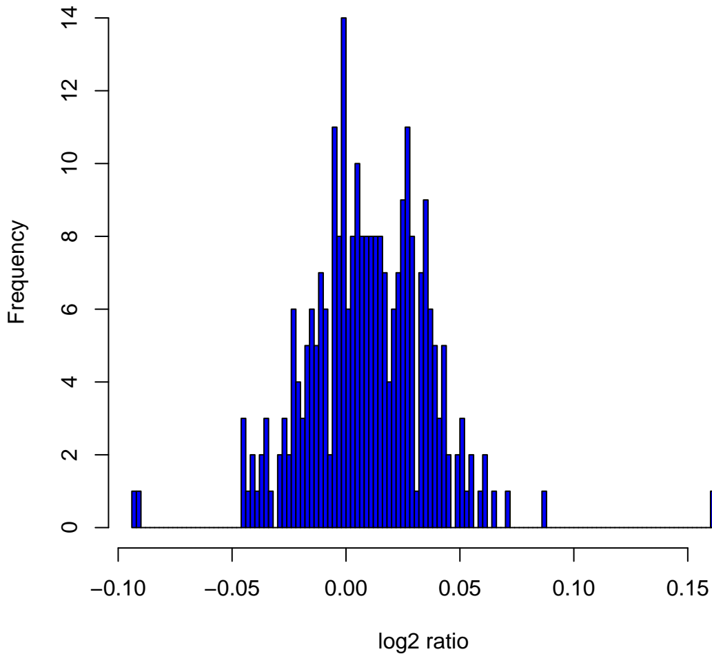
Histogram of log 2 ratios in 270 HapMap samples at clone Chr19tp-1B7
