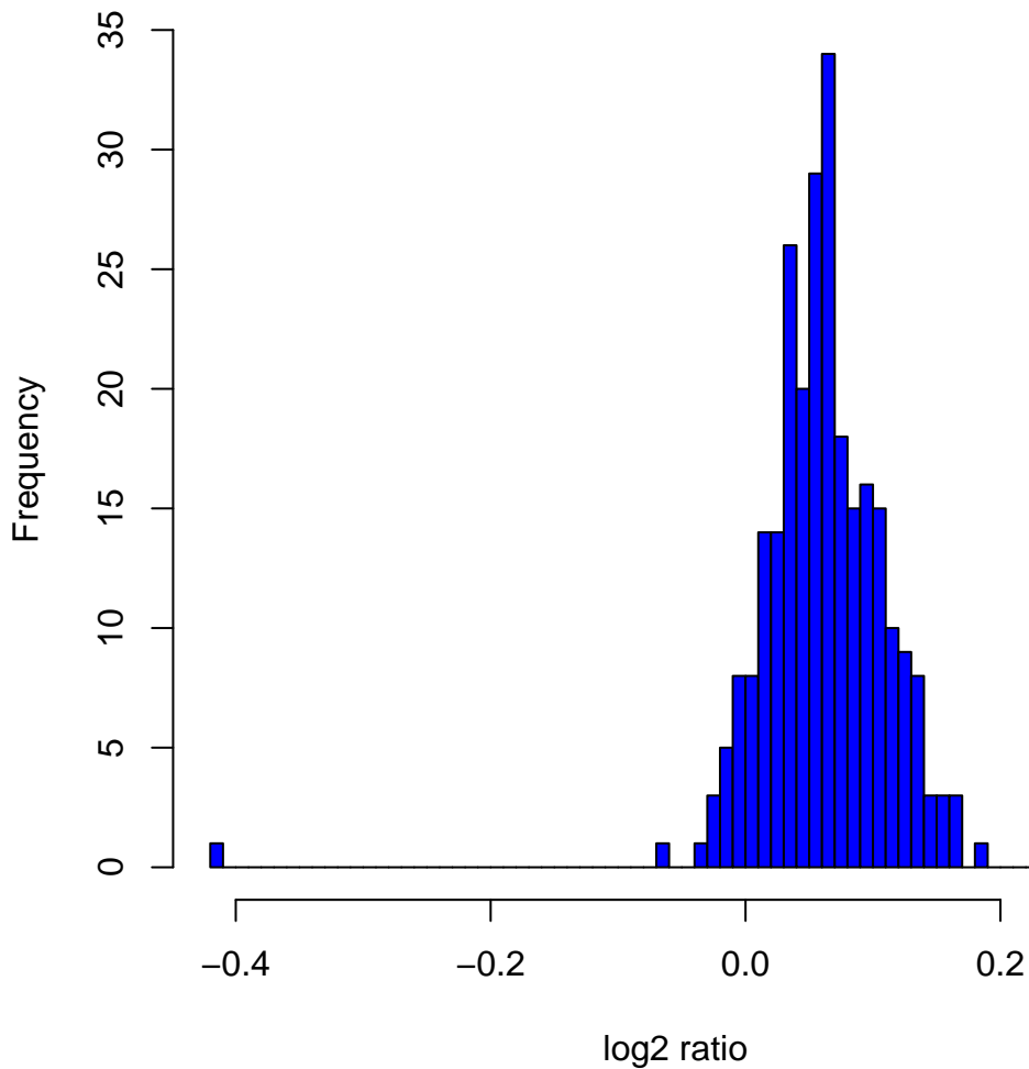
Histogram of log 2 ratios in 270 HapMap samples at clone Chr19tp-2C4
