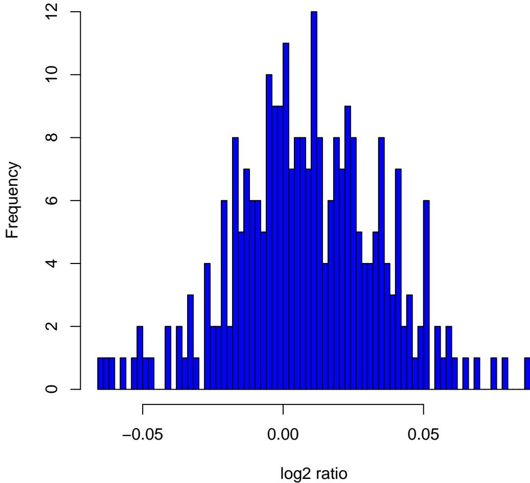
Histogram of log2ratios in 270 HapMap samples at clone Chr19tp-4A2
