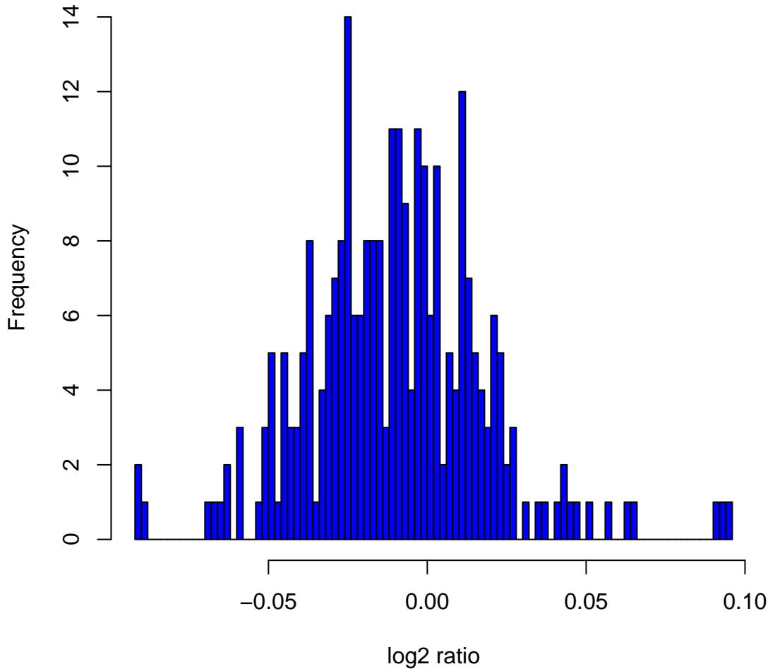
Histogram of log 2 ratios in 270 HapMap samples at clone Chr19tp-4C8
