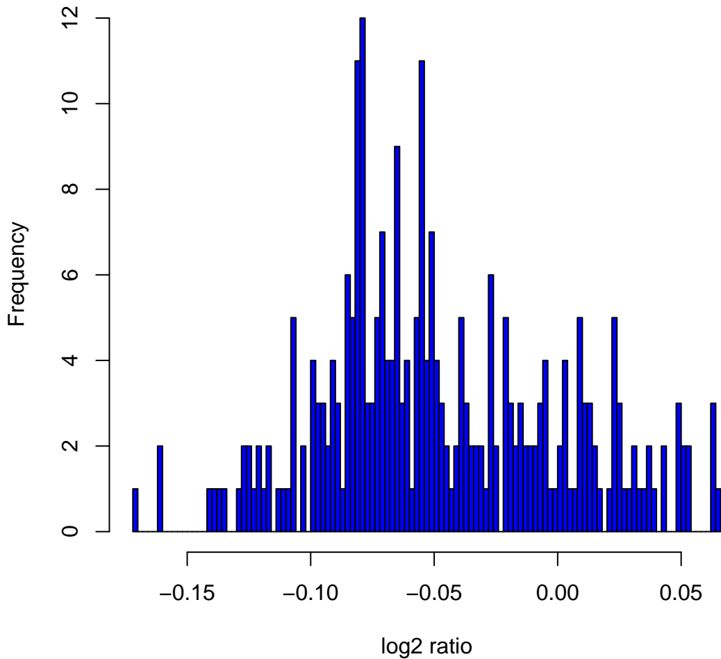
Histogram of log2ratios in 270 HapMap samples at clone Chr19tp-4D12
