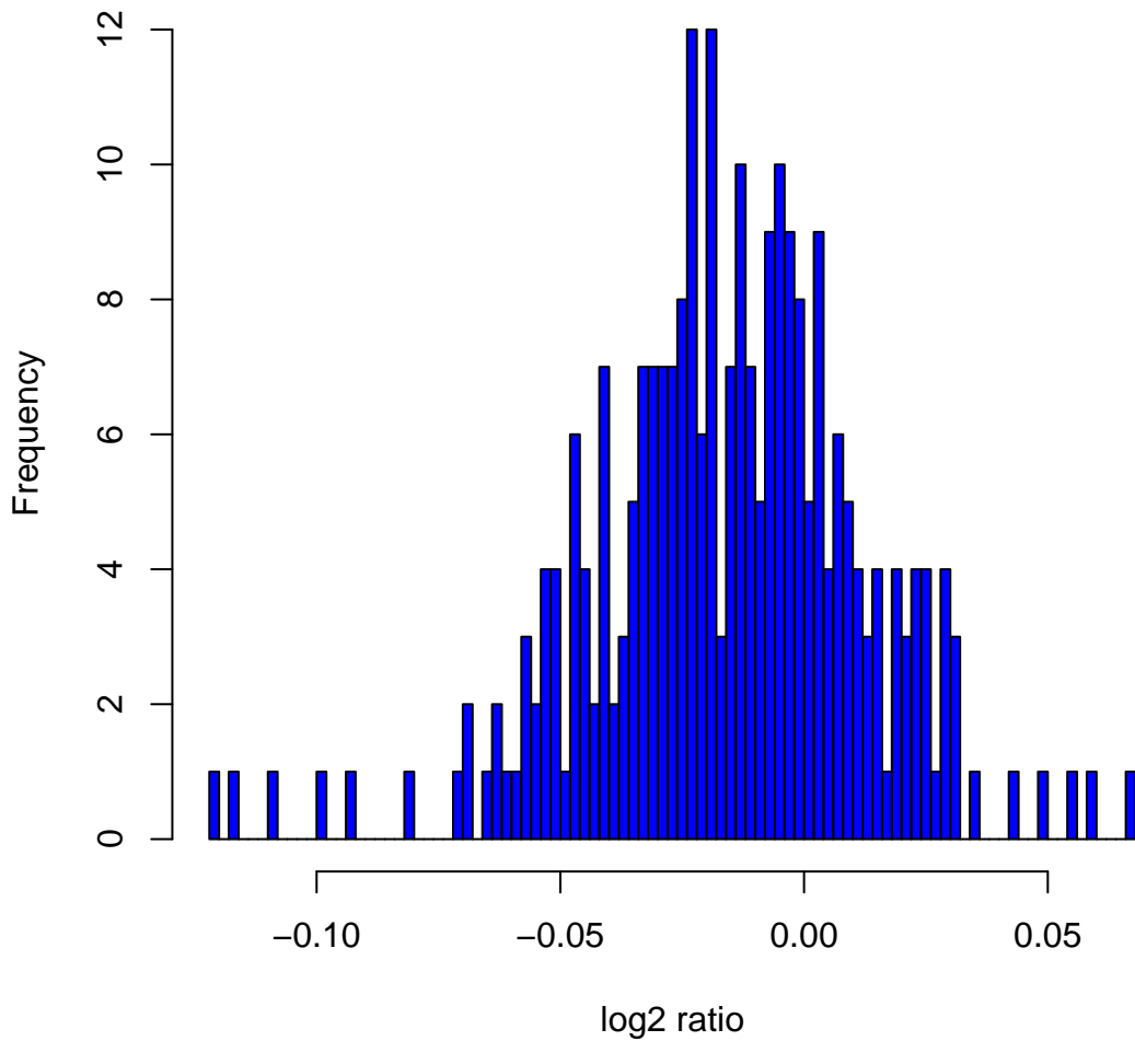
Histogram of log 2 ratios in 270 HapMap samples at clone Chr19tp-4D6
