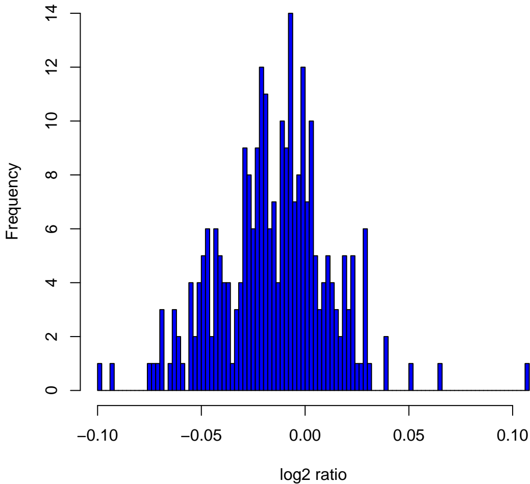
Histogram of log2ratios in 270 HapMap samples at clone Chr19tp-6A10
