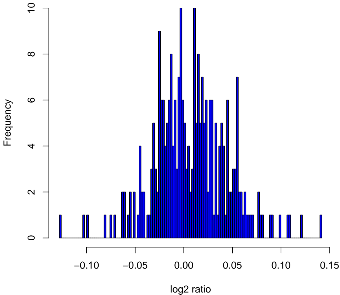
Histogram of log2ratios in 270 HapMap samples at clone Chr19tp-6A12
