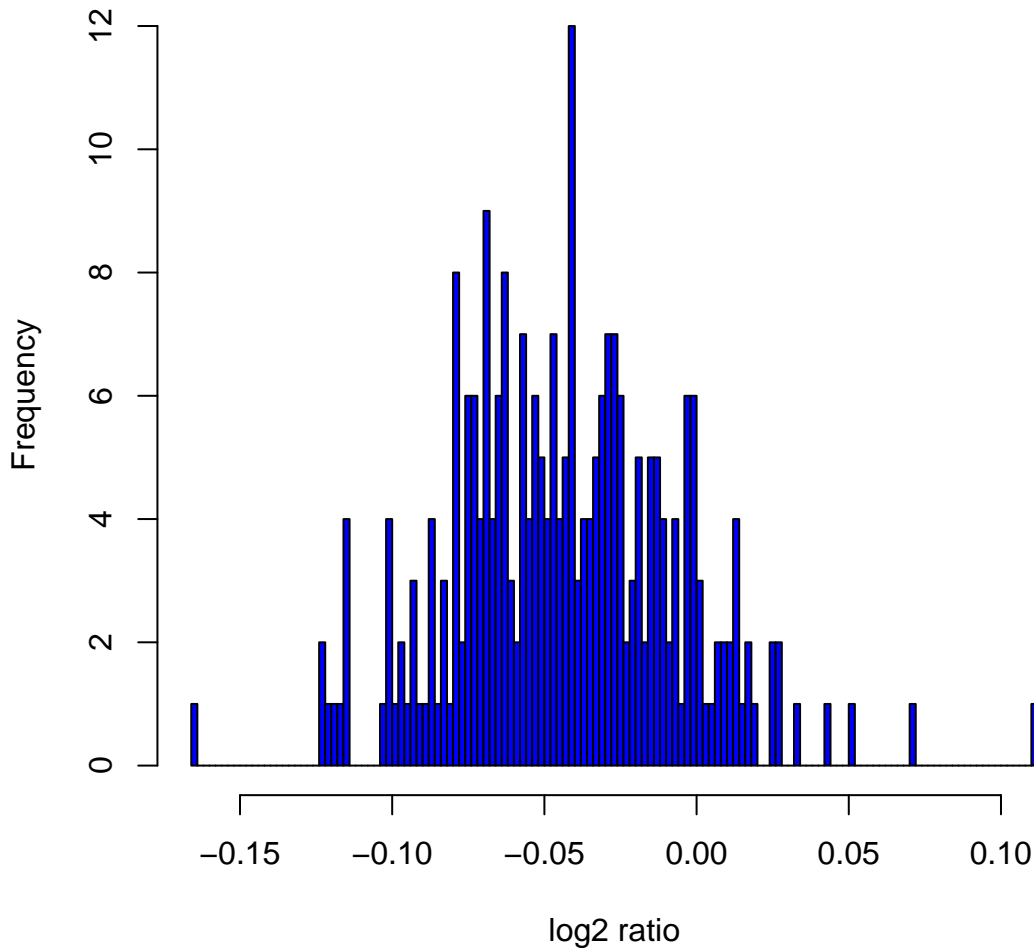
Histogram of log 2 ratios in 270 HapMap samples at clone Chr19tp-6B2
