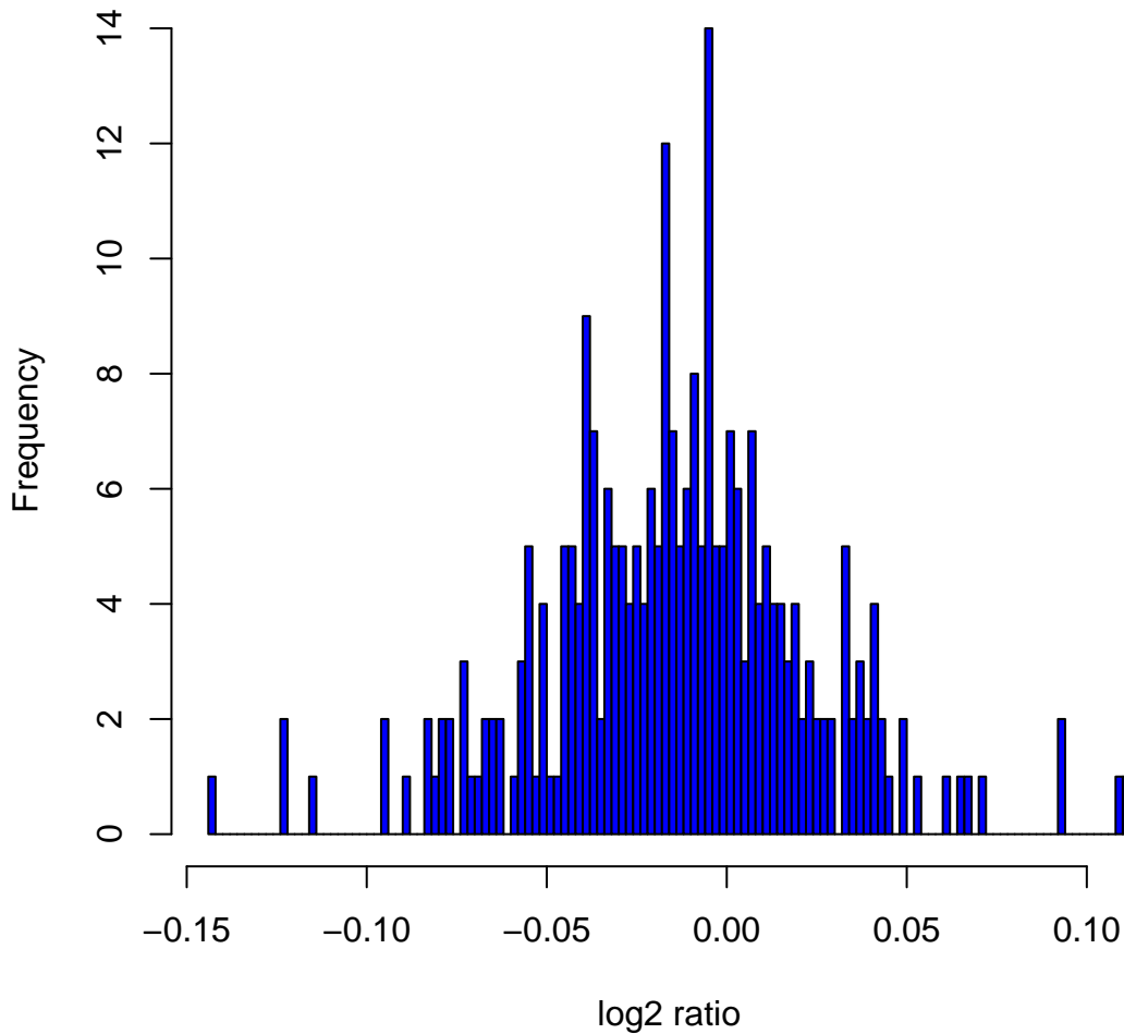
Histogram of \log_2 ratios in 270 HapMap samples at clone Chr19tp-6B6
