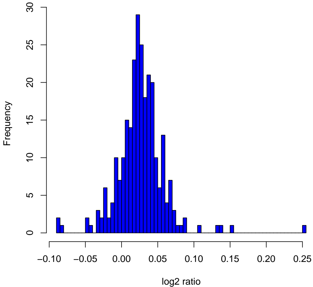
Histogram of log2ratios in 270 HapMap samples at clone Chr19tp-6C11
