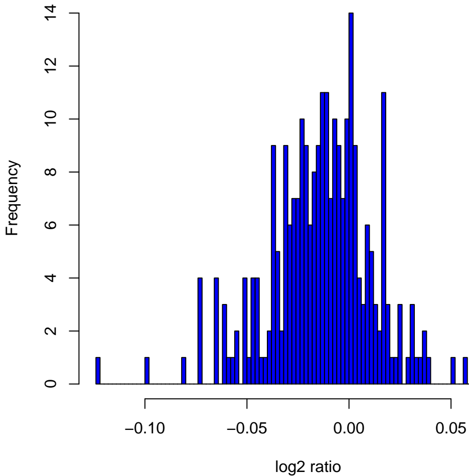
Histogram of log 2 ratios in 270 HapMap samples at clone Chr19tp-6C7
