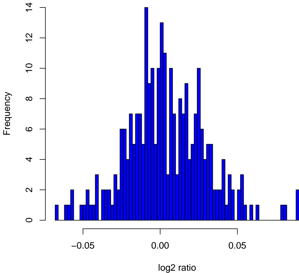
Histogram of log 2 ratios in 270 HapMap samples at clone Chr19tp-6E1
