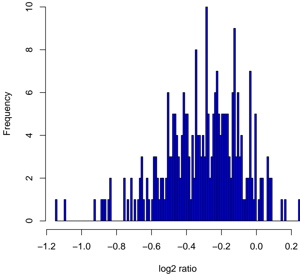
Histogram of log2ratios in 270 HapMap samples at clone Chr19tp-6H5
