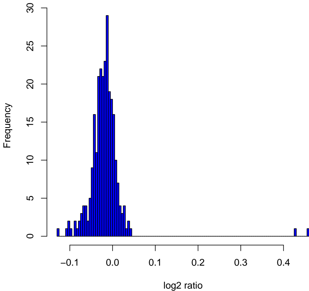
Histogram of log 2 ratios in 270 HapMap samples at clone Chr19tp-7D9
