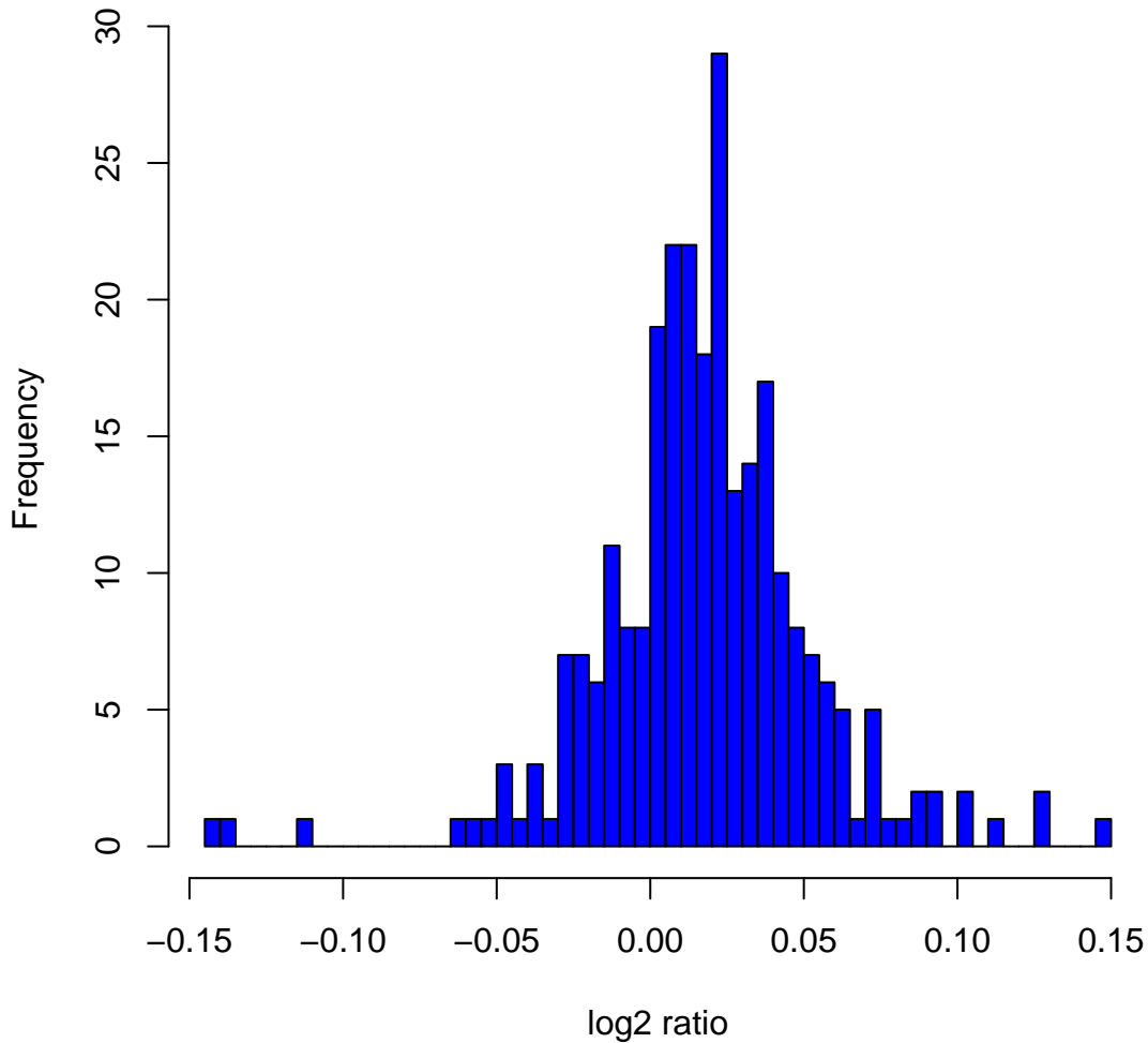
Histogram of log 2 ratios in 270 HapMap samples at clone Chr20tp-1C1
