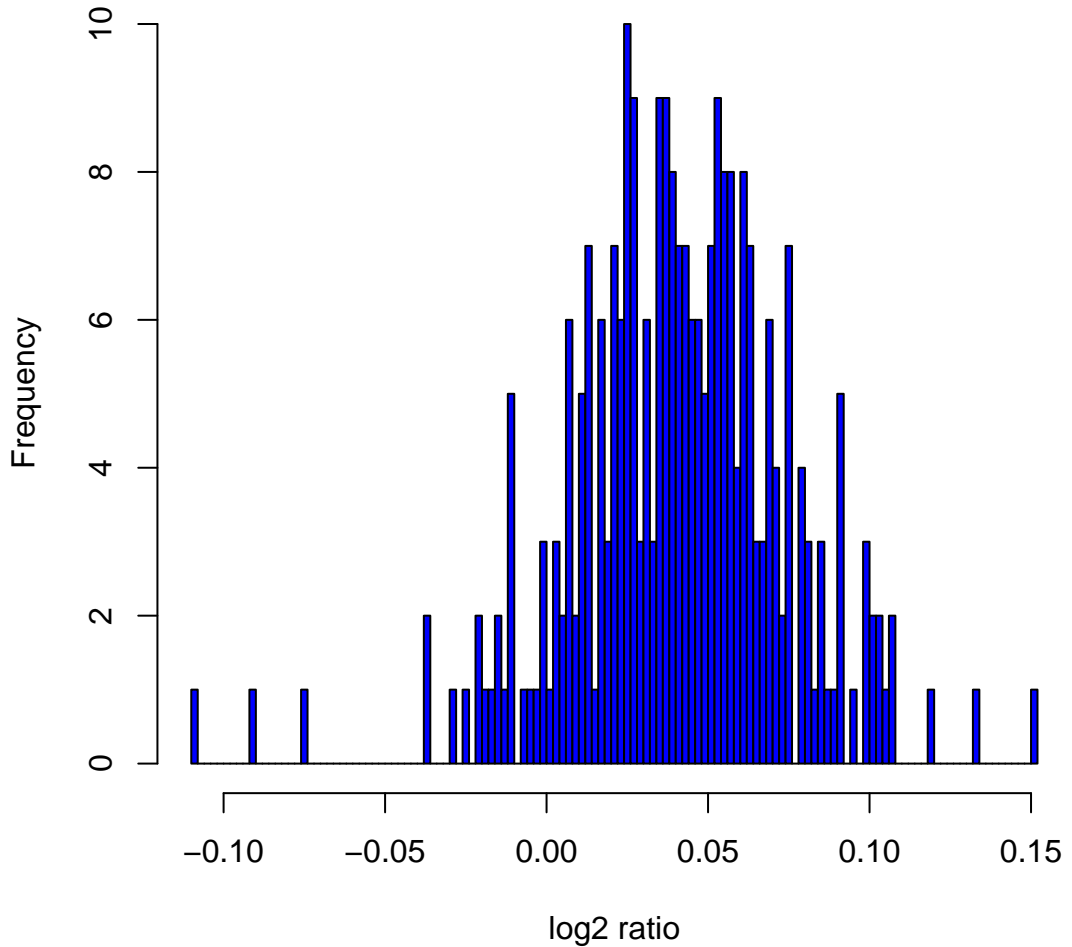
Histogram of log 2 ratios in 270 HapMap samples at clone Chr20tp-1C4
