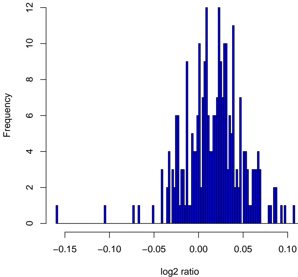
Histogram of log 2 ratios in 270 HapMap samples at clone Chr20tp-1D1
