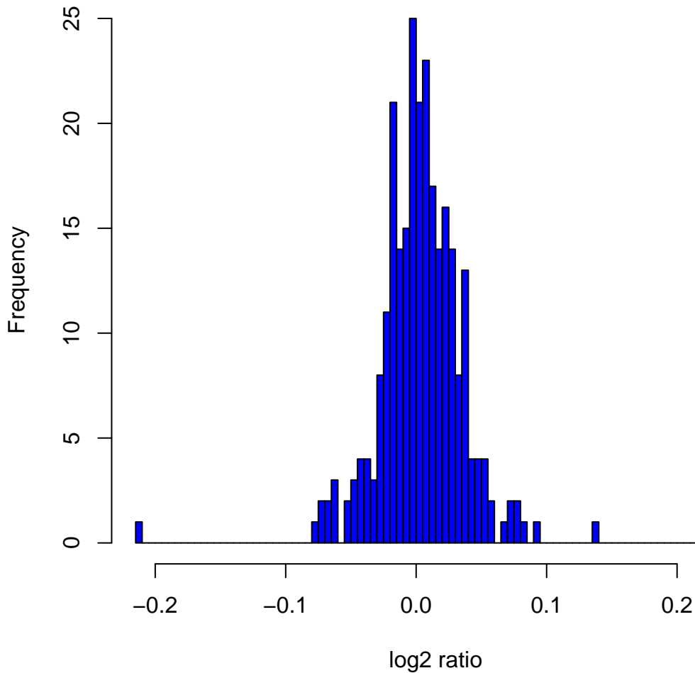
Histogram of log2ratios in 270 HapMap samples at clone Chr20tp-1E10
