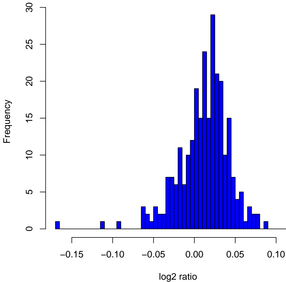
Histogram of log2ratios in 270 HapMap samples at clone Chr20tp-1F11
