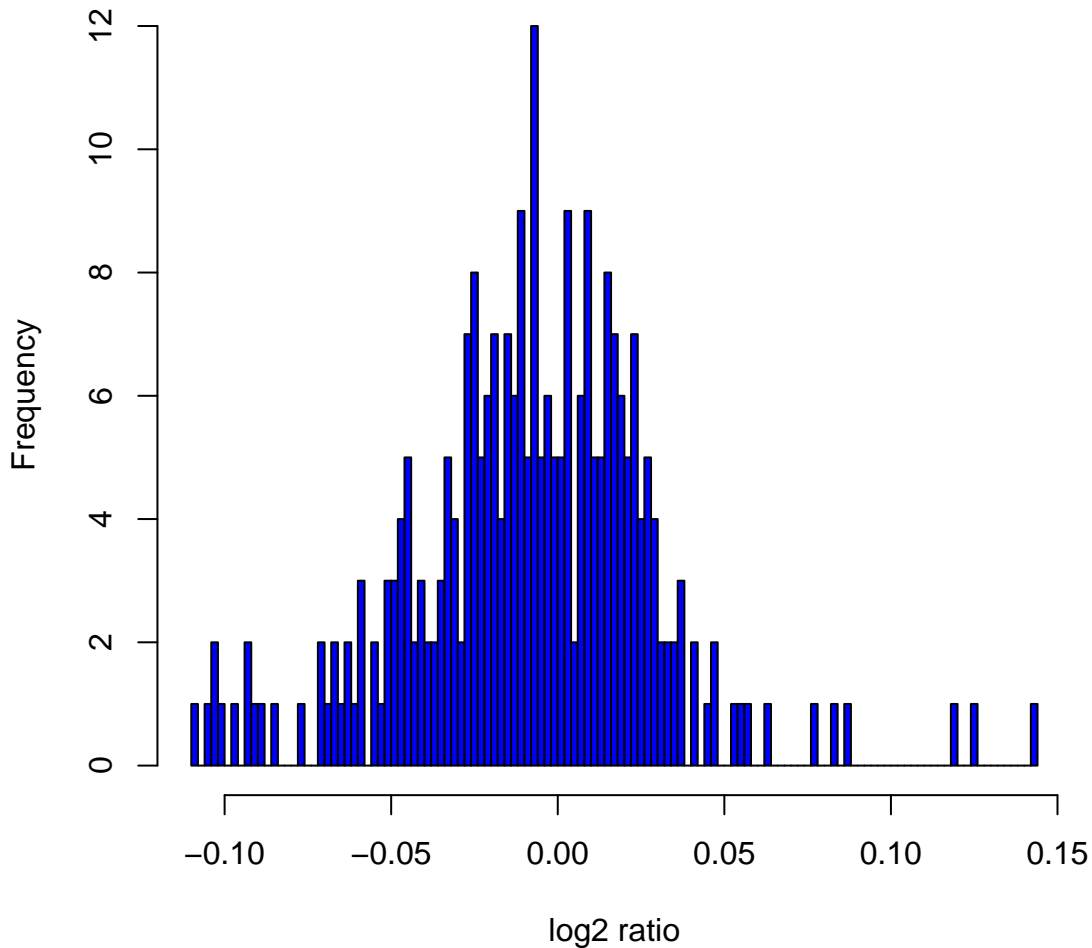
Histogram of log2ratios in 270 HapMap samples at clone Chr20tp-2A10
