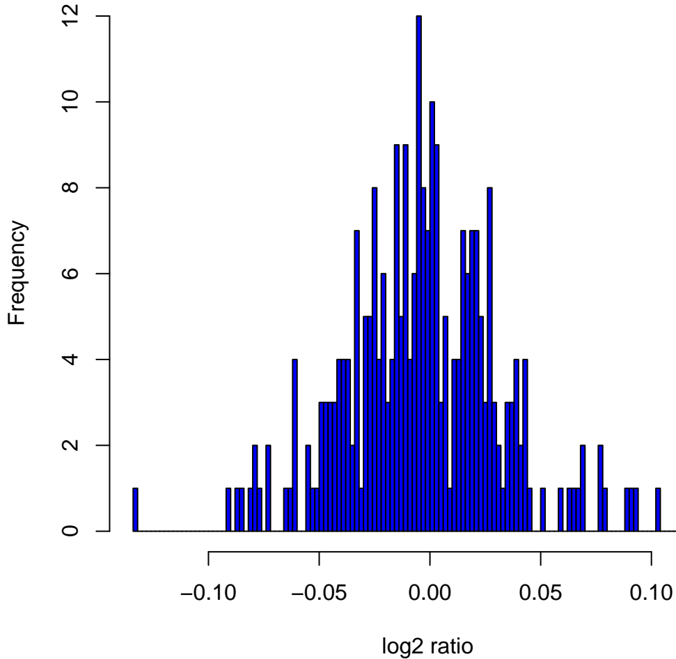
Histogram of log2ratios in 270 HapMap samples at clone Chr20tp-2B5
