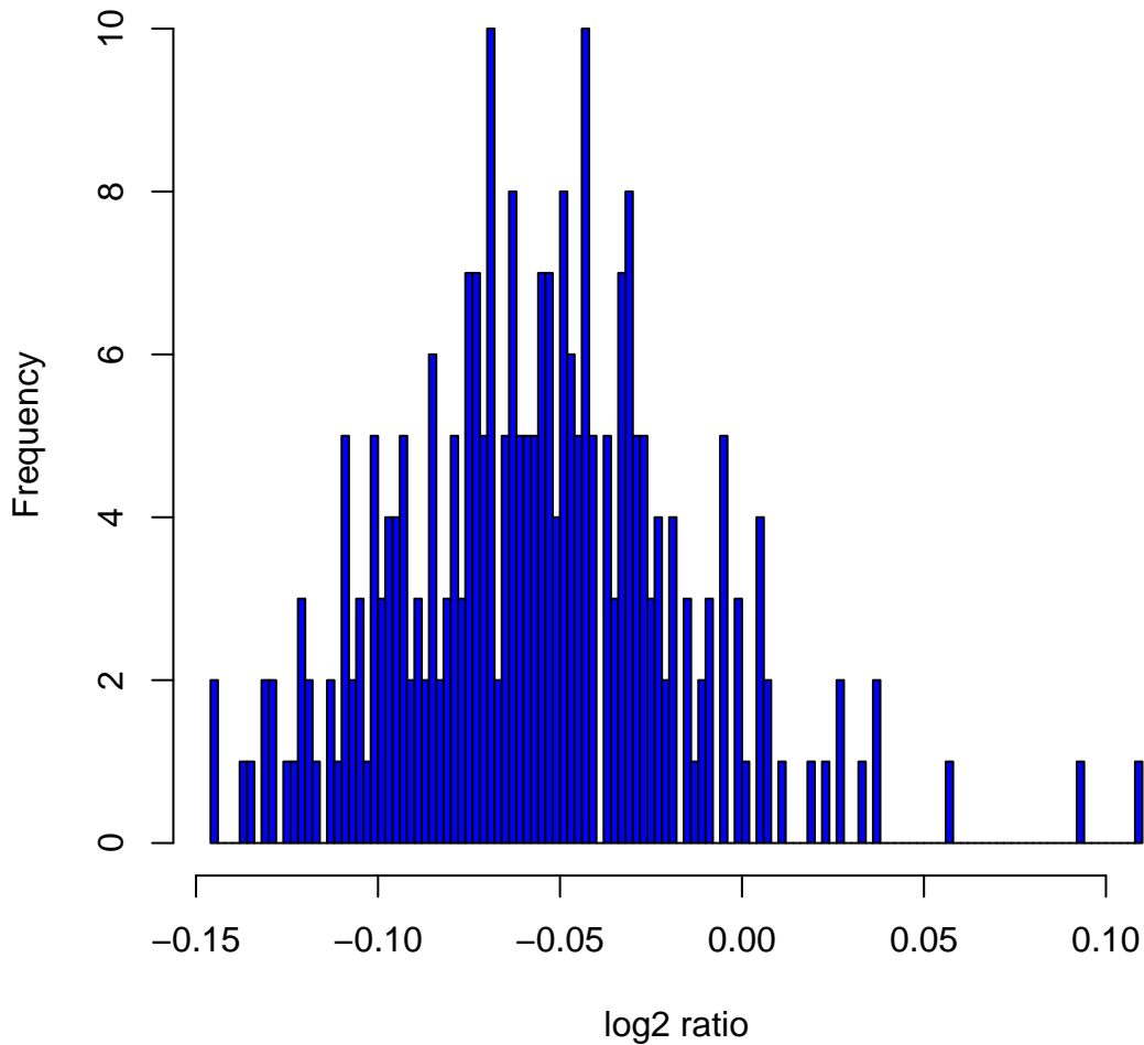
Histogram of log 2 ratios in 270 HapMap samples at clone Chr20tp-2C1
