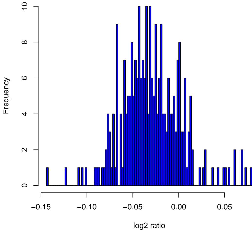
Histogram of log2ratios in 270 HapMap samples at clone Chr20tp-2C12
