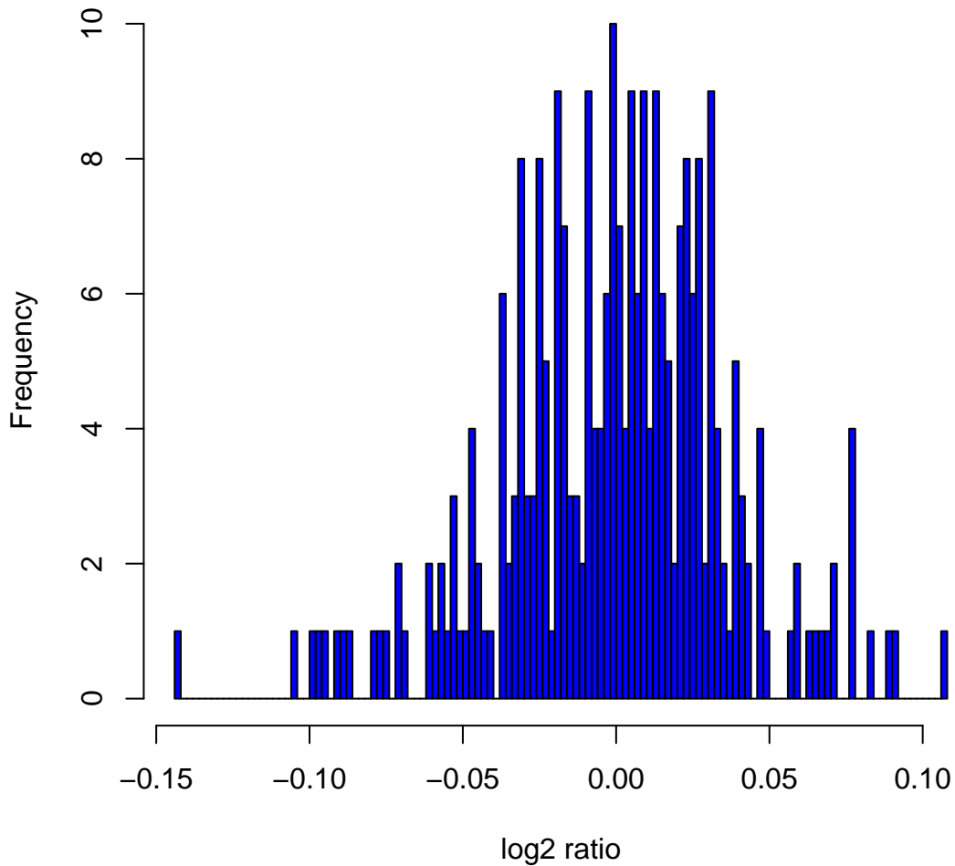
Histogram of log 2 ratios in 270 HapMap samples at clone Chr20tp-2G1
