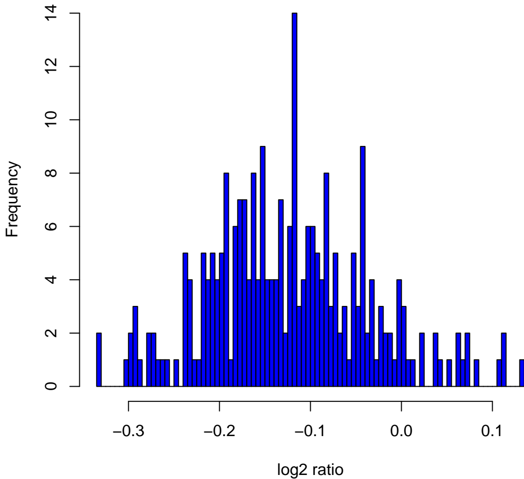
Histogram of log2ratios in 270 HapMap samples at clone Chr20tp-2G12
